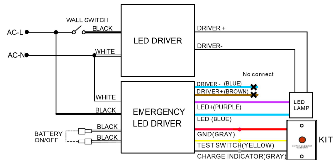
Wiring Diagram 1 (When driver power is more than 100W)
