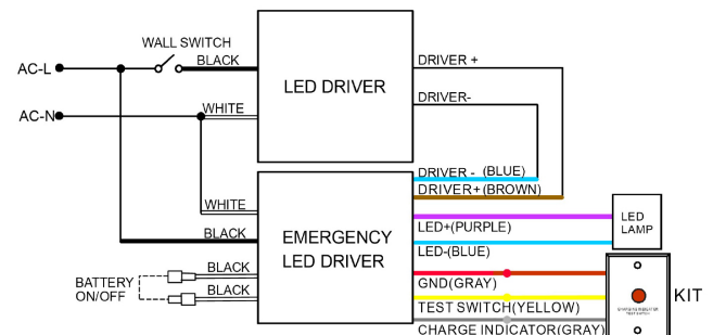
Wiring Diagram 2 (When driver power is less than 100W)
